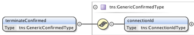
Figure 56 – terminateConfirmed message structure.
