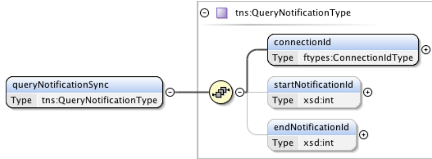
Figure 80 – queryNotificationSync request message structure.
