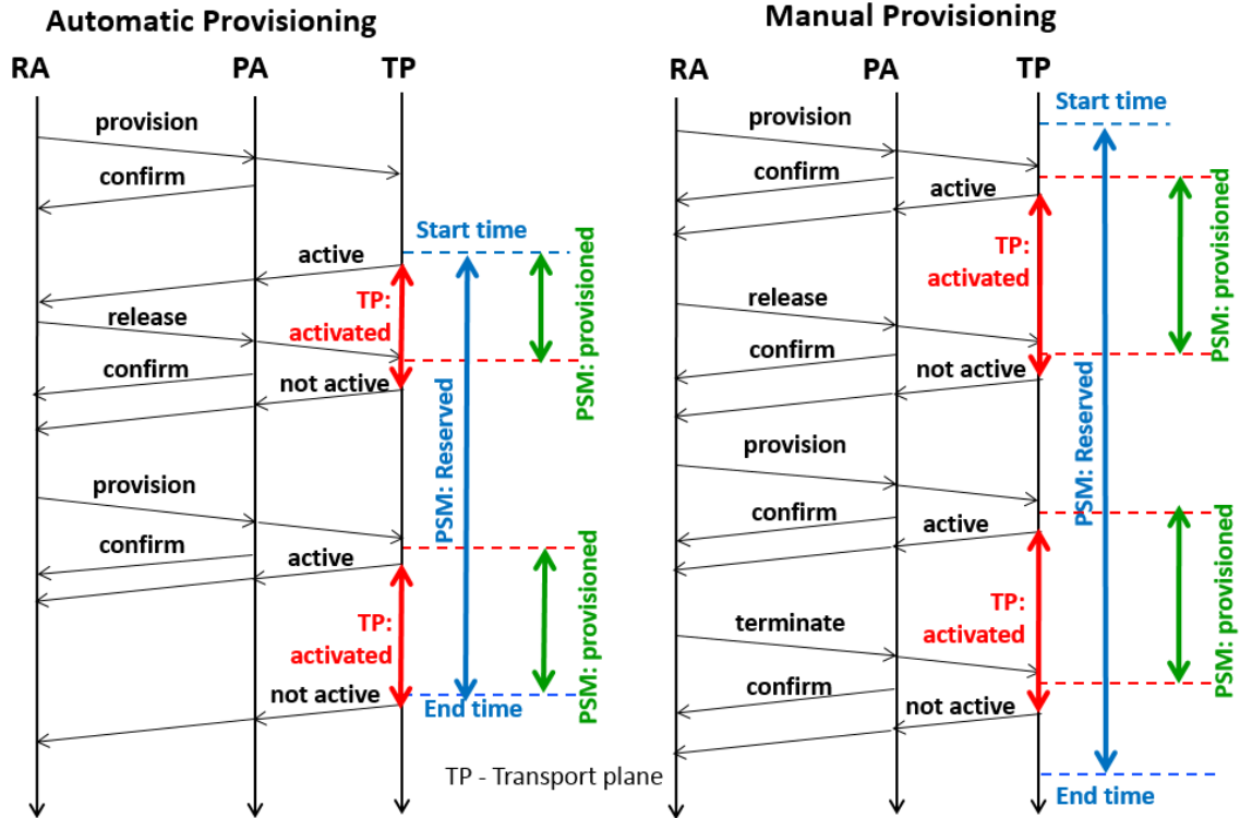
Figure 8: Release and Provisioning
