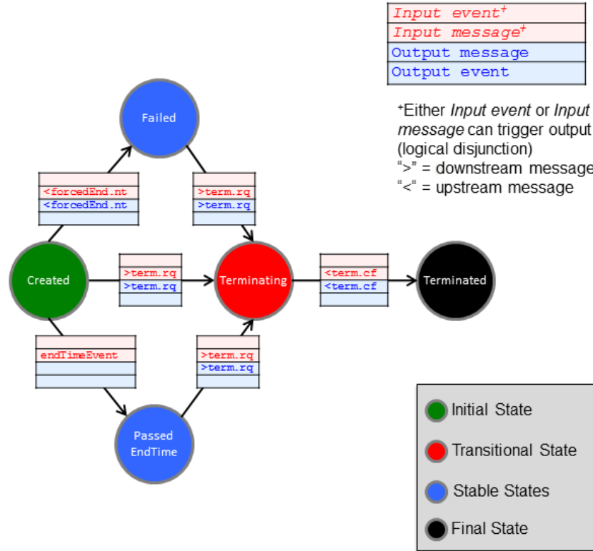
Figure 5: Lifecycle State Machine
