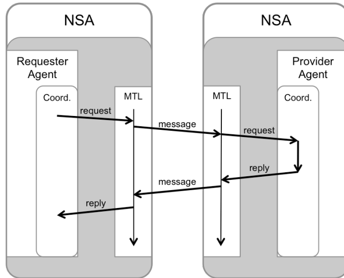
Figure 10: Synchronous messages and MTL and Coordinator functions.
