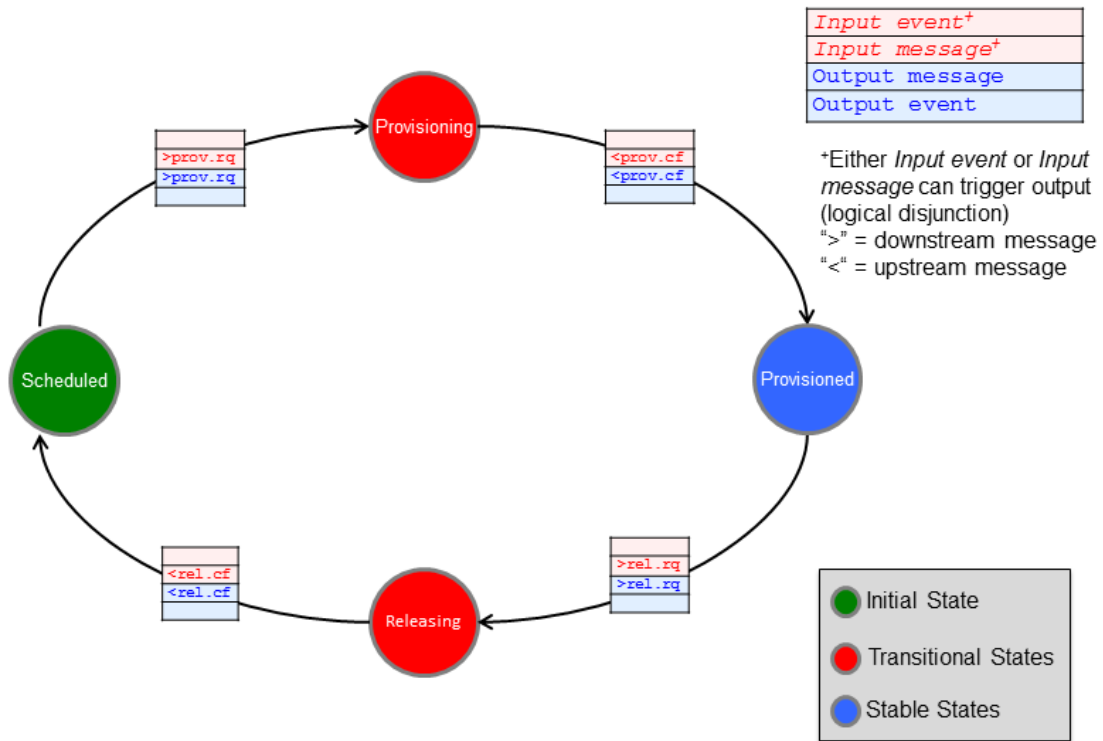
Figure 4: Provision State Machine
