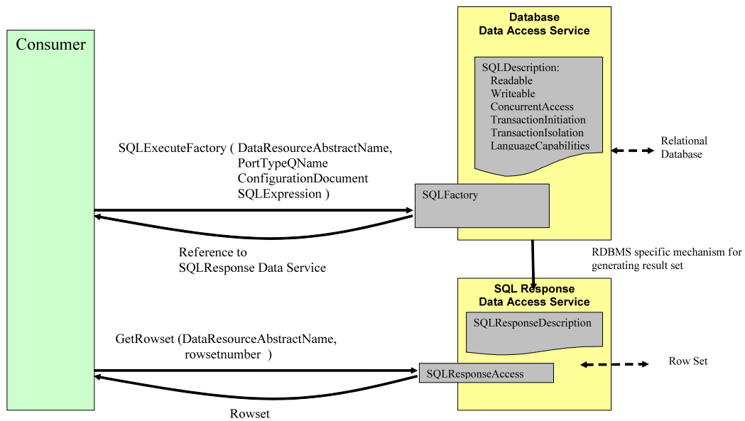
Figure 4: Data factory example based on WS-DAIR realization
