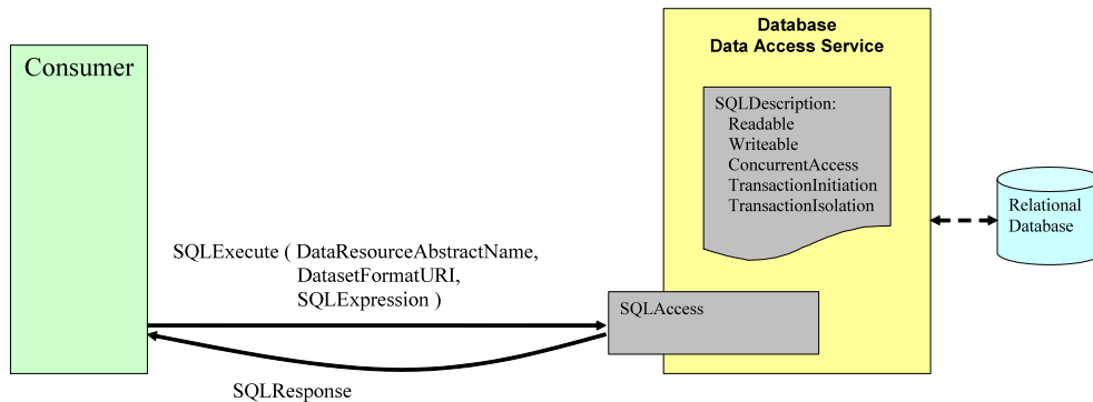
Figure 3: Data access example based on the WS-DAIR realization
