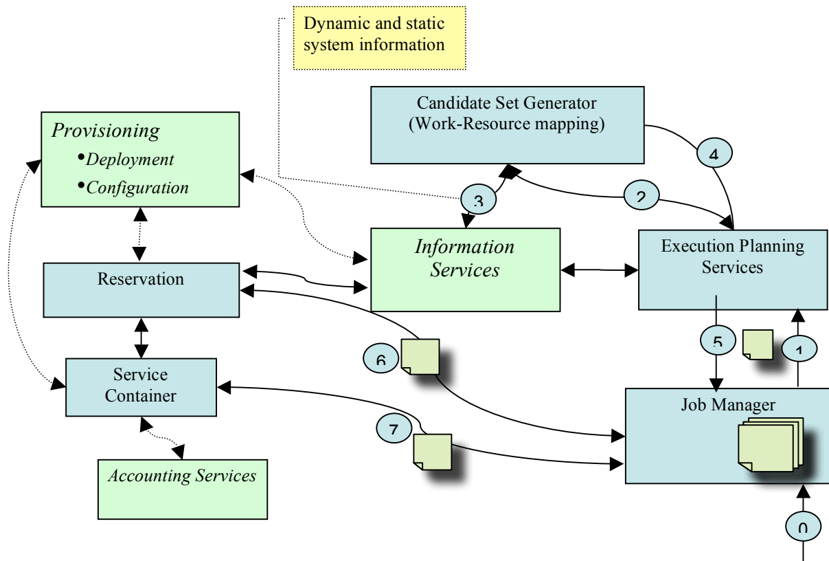
Figure 4: Interactions of EMS services to execute a legacy BLAST job
