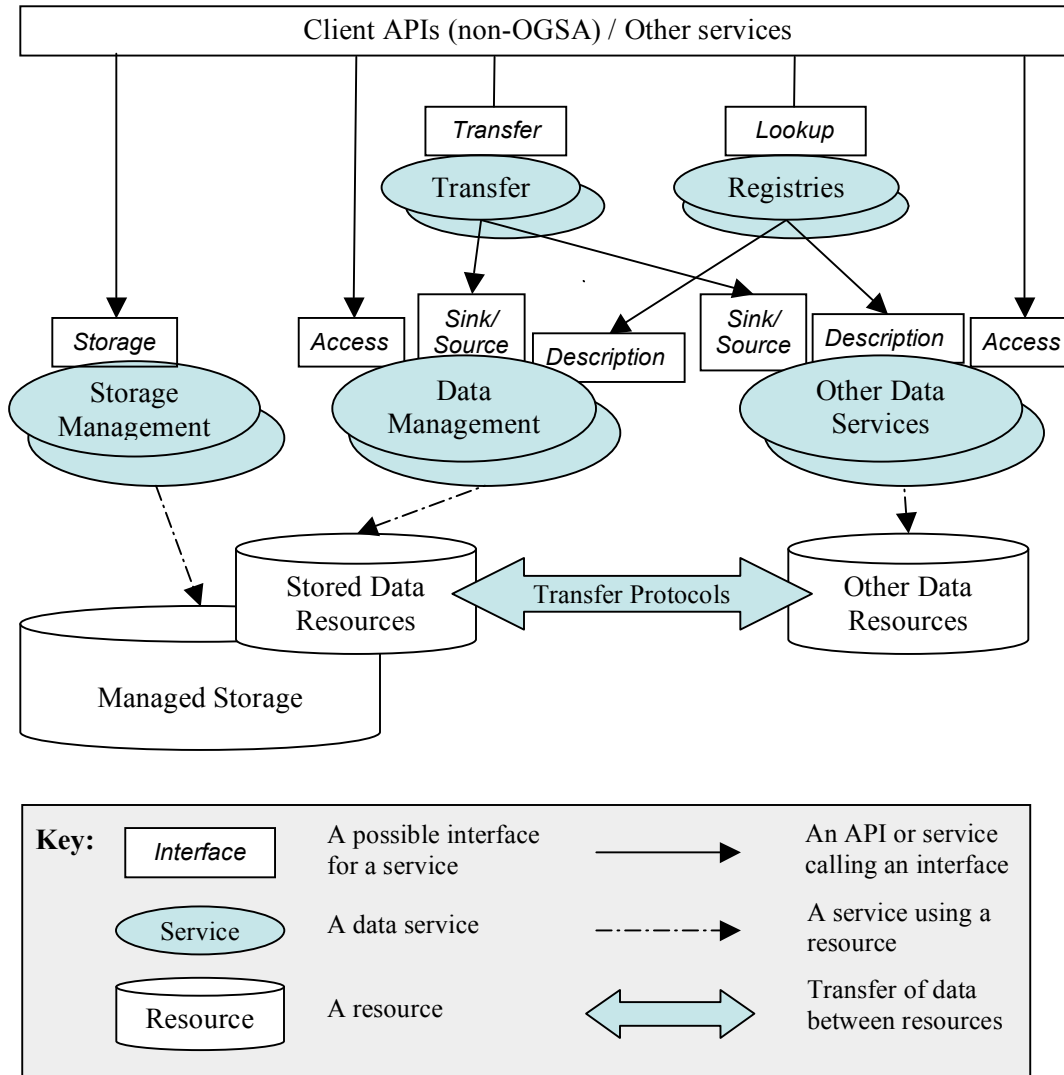
Figure 5: Basic entities in the data architecture
