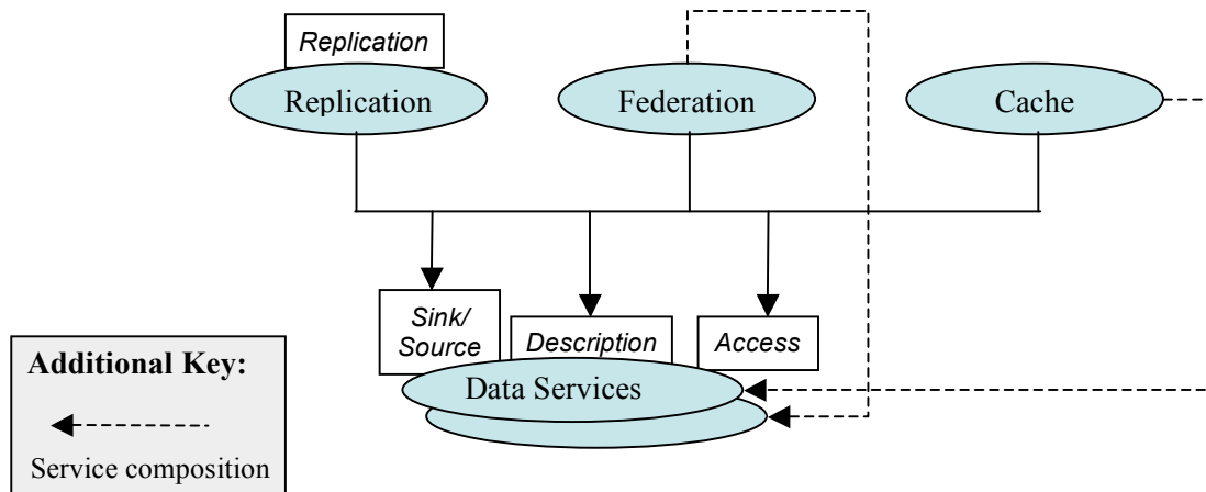
Figure 6: Composite entities in the data architecture
